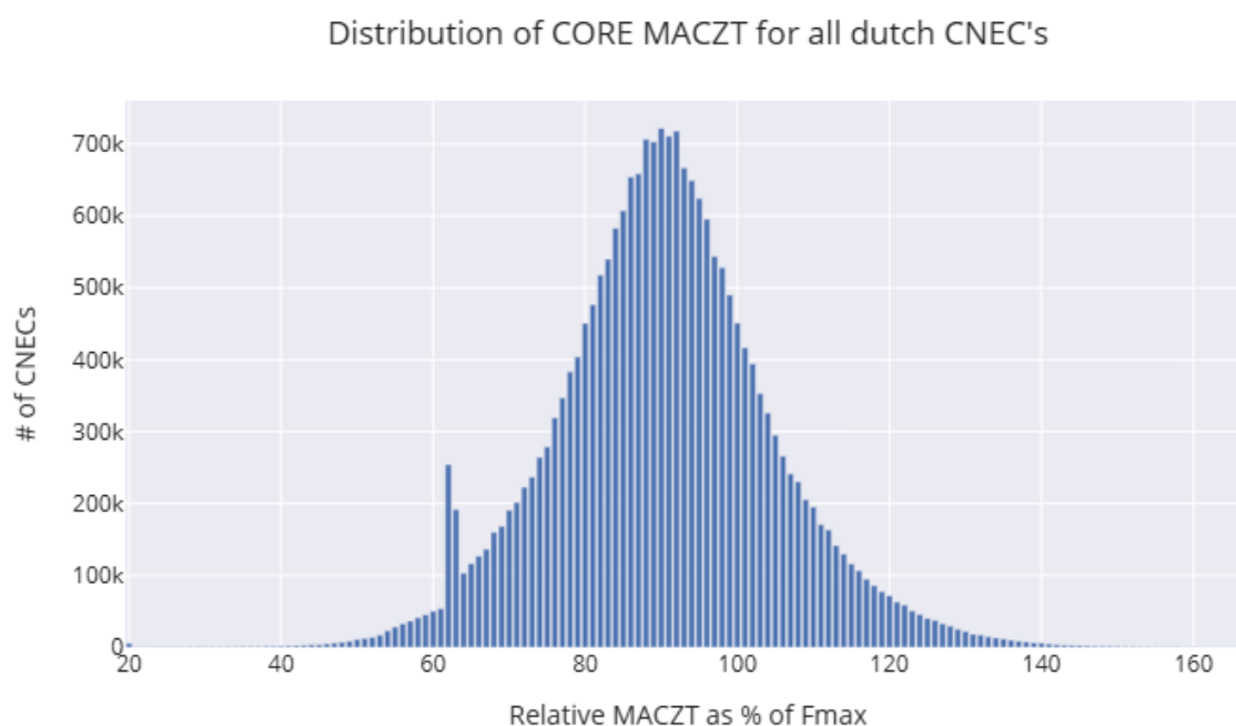
Figure 6: Distribution of the relative MACZT for all CNECs and hours of the Netherlands for the Core CCR.
