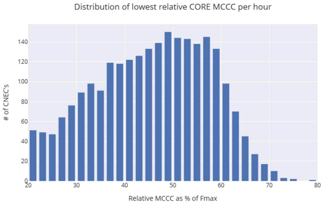
Figure 4: Distribution of the lowest hourly relative MCCC of the Netherlands for the Core CCR.
