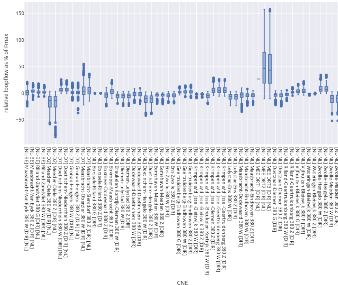
Figure 12: Average relative loop flow per Dutch CNE per hour. Positive values indicate loop flows in the forward direction, negative values indicate loop flows in the opposite direction.
