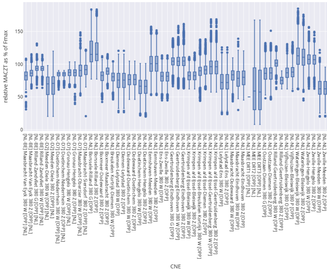
Relative MACZT per Dutch CNE for CORE, minimum per hour, opposite direction
