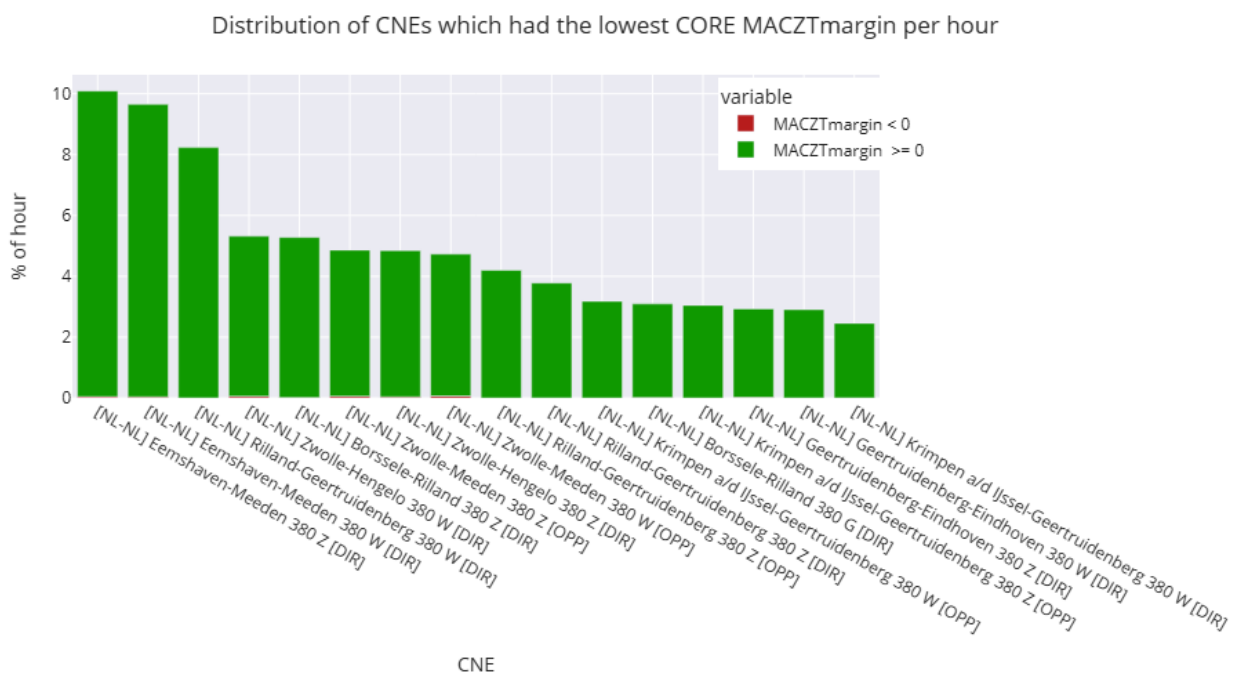
Figure 10: Overview of least performing CNEs in Core CCR w.r.t. MACZT_{margin} . It has been determined what percentage of time an individual CNE has been the CNEC with the lowest MACZT_{margin} per hour. The green part of the bar indicates the percentage of time that the CNE had a positive MACZT_{margin} the red part indicates the time that the CNE had a MACZT_{margin} < 0 . All CNEs occurring <1% of the time are excluded from the graph.
