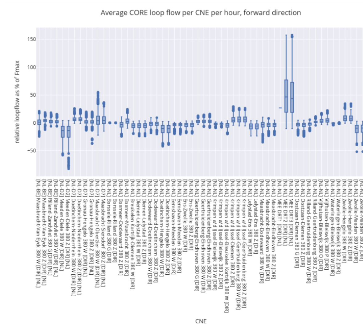
Figure 1: Average relative loop flow per Dutch CNE per MTU. Positive values indicate loop flows in the forward direction, negative values indicate loop flows in the opposite direction. CORE CCR, considering third countries. Period Jan 1 - Dec 31, 2025
