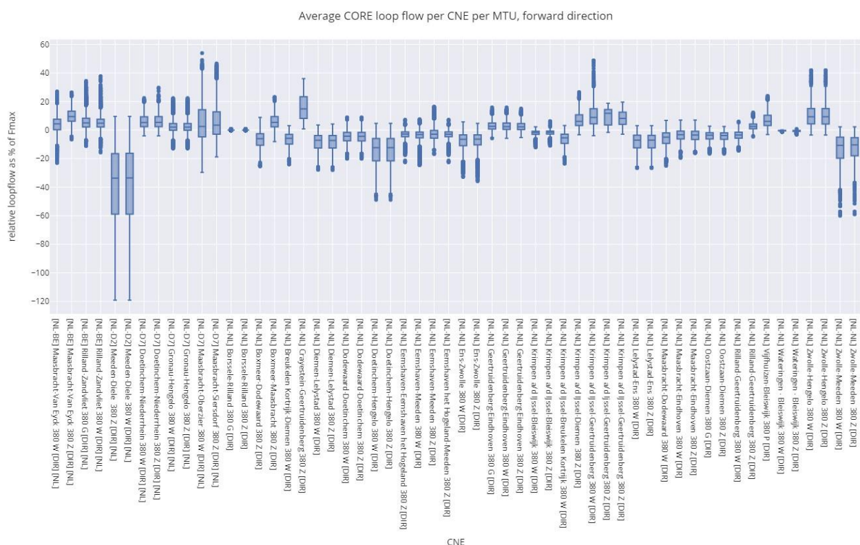
Figure 1: Average relative loop flow per Dutch CNE per MTU. Positive values indicate loop flows in the forward direction, negative values indicate loop flows in the opposite direction. CORE CCR, considering third countries. Period Jan 1 - Dec 31, 2023
