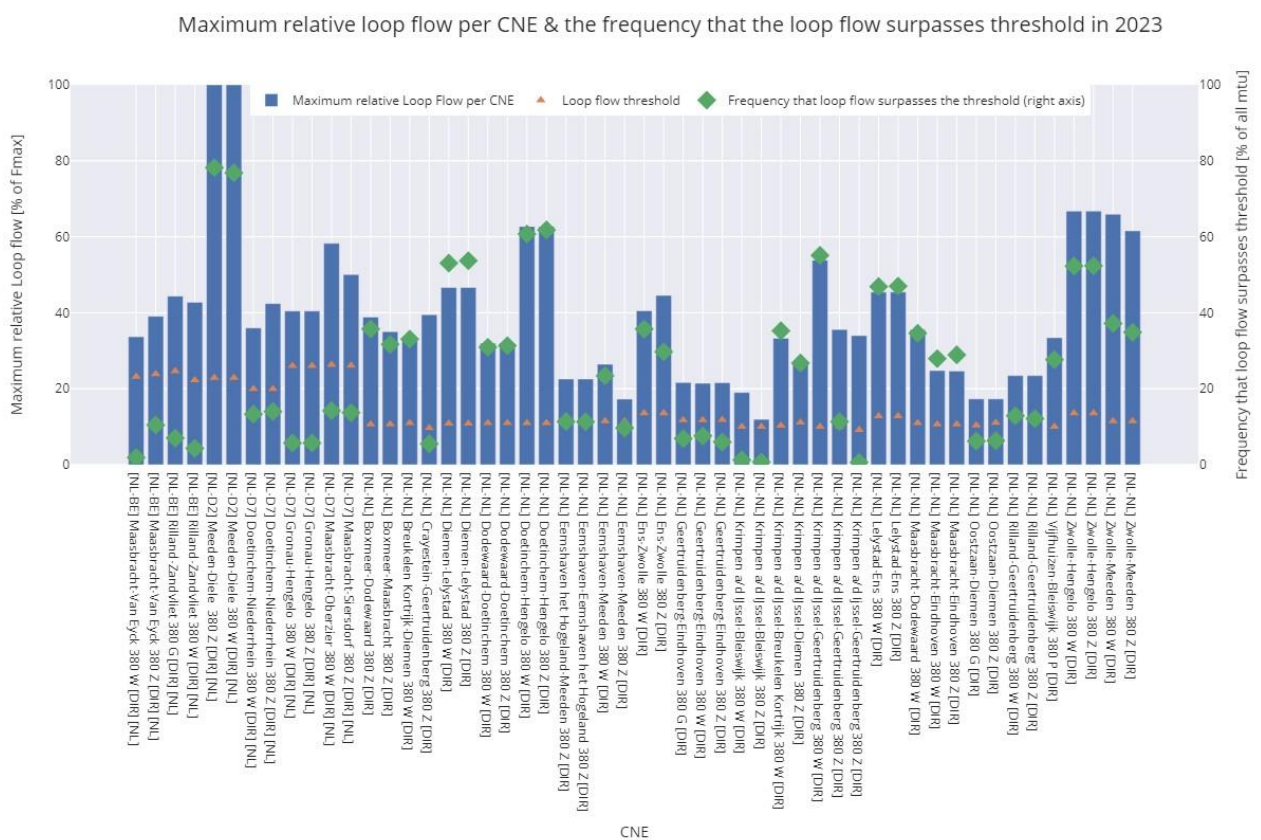
Figure 2: Maximum relative loop flow per Dutch CNE and the frequency for which the loop flow surpassed the threshold. CORE CCR, considering third countries. Period Jan 1 - Dec 31, 2023
