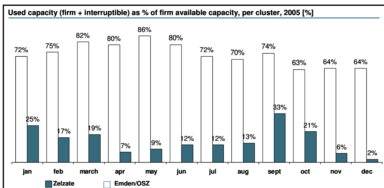
Figure 6. Use of import capacity per cluster in 2005. Source: GTS
