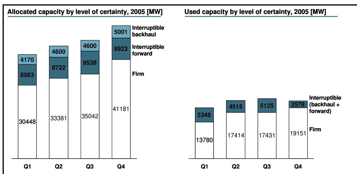
figure 5. Reserved and used interruptible capacity and firm import capacity for H Gas. Source: GTS
