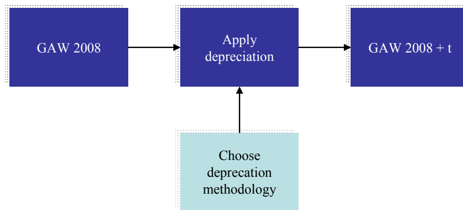
Figure 2: Determining the GAW-GA from 2008
