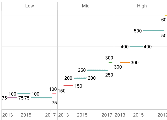
Upload (Mbps)
